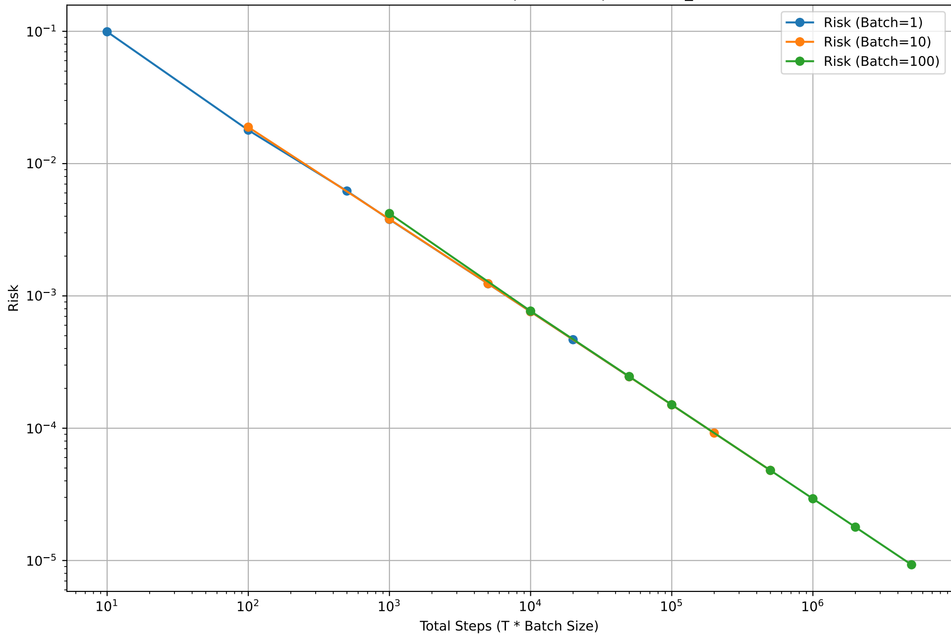
Slock Risk for Different Batch Sizes; \alpha=2.5 . optiized eta_star for each T
